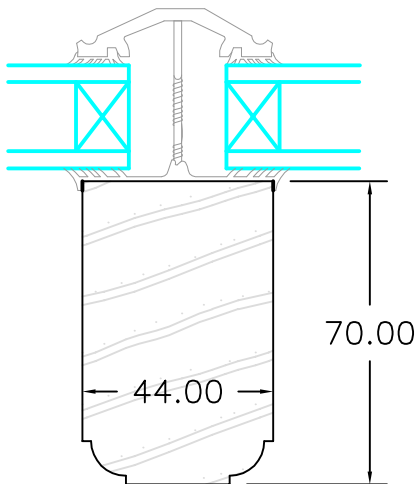
Rafter.
