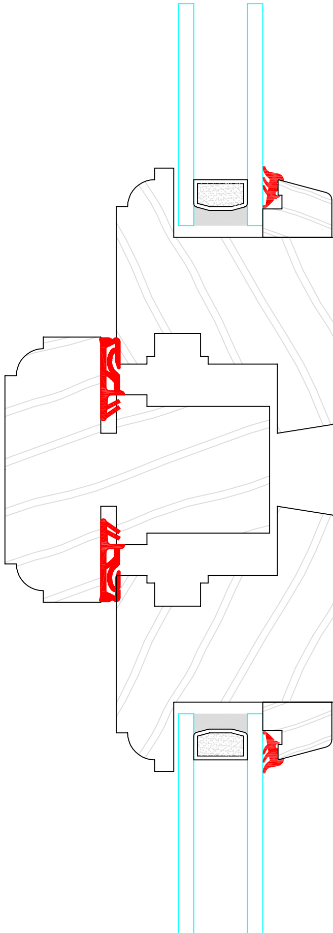
HP Storm mullion and transom section - 9 dig splay moulding
