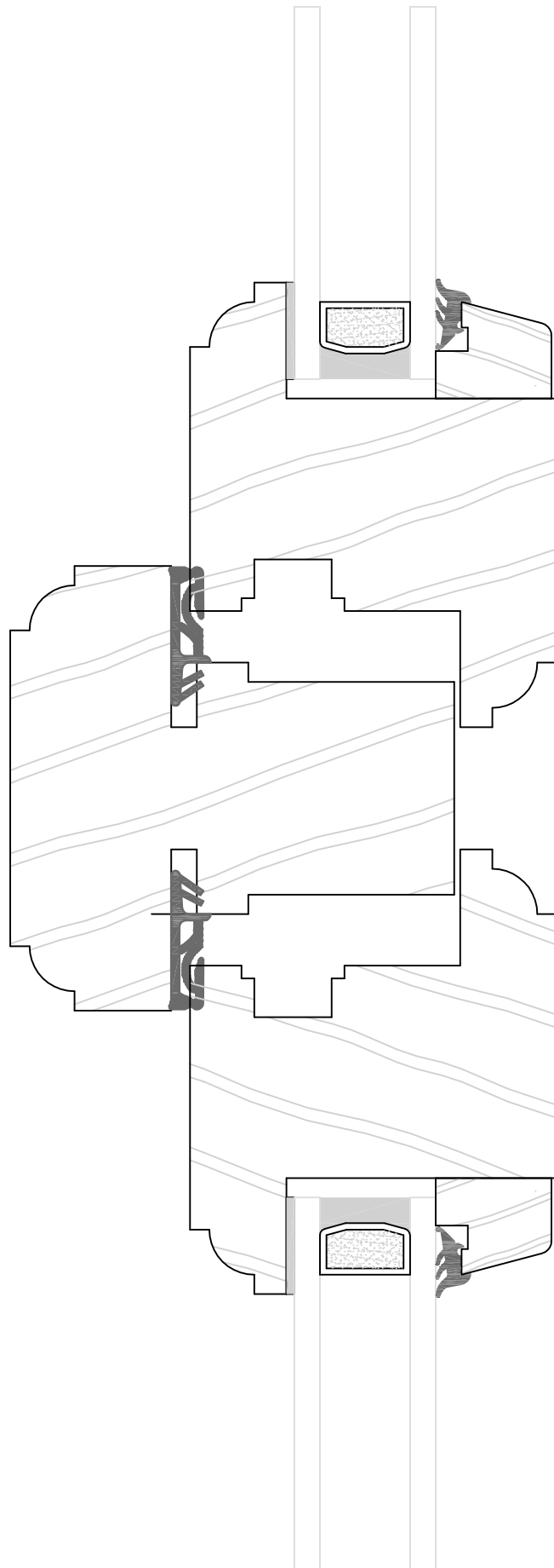
HP Storm transom and mullion section - Ovolo moulding
